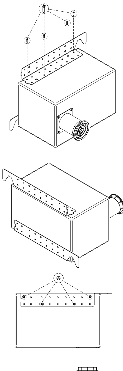
Figure 2: diagram of wall installation
