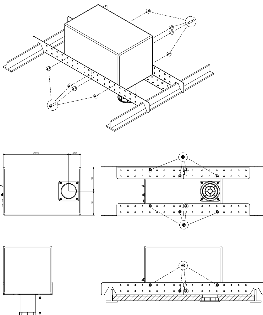
Figure 1: diagram for suspended ceiling installation
